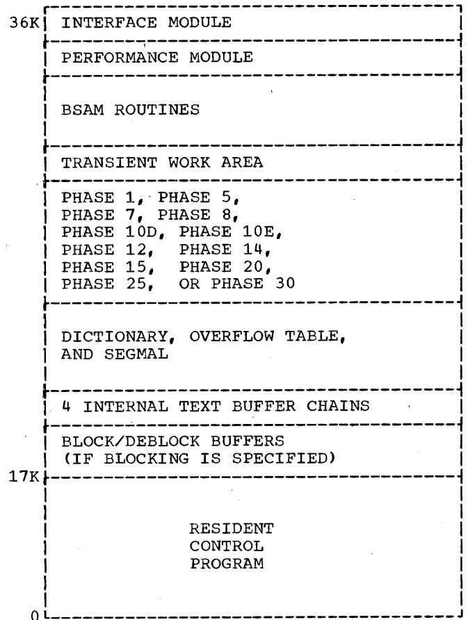
Figure 23. Main Storage Allocation for a PRFRM Compilation
